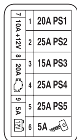
Fuse Box and Cover
