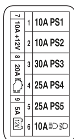
Fuse Box and Cover
